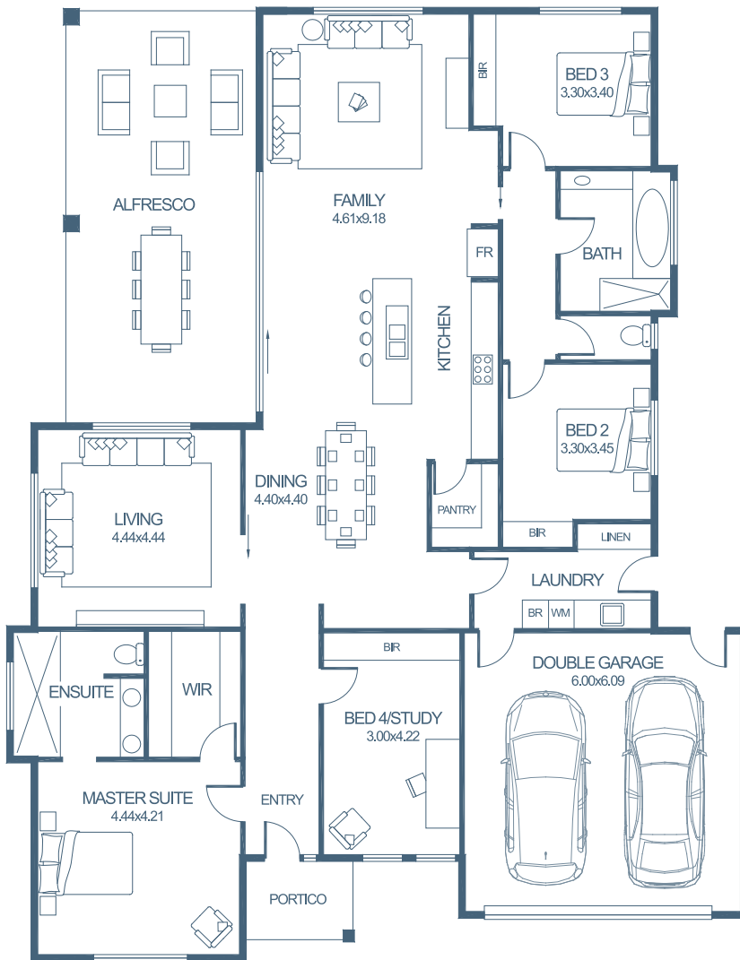
FLOORPLAN
