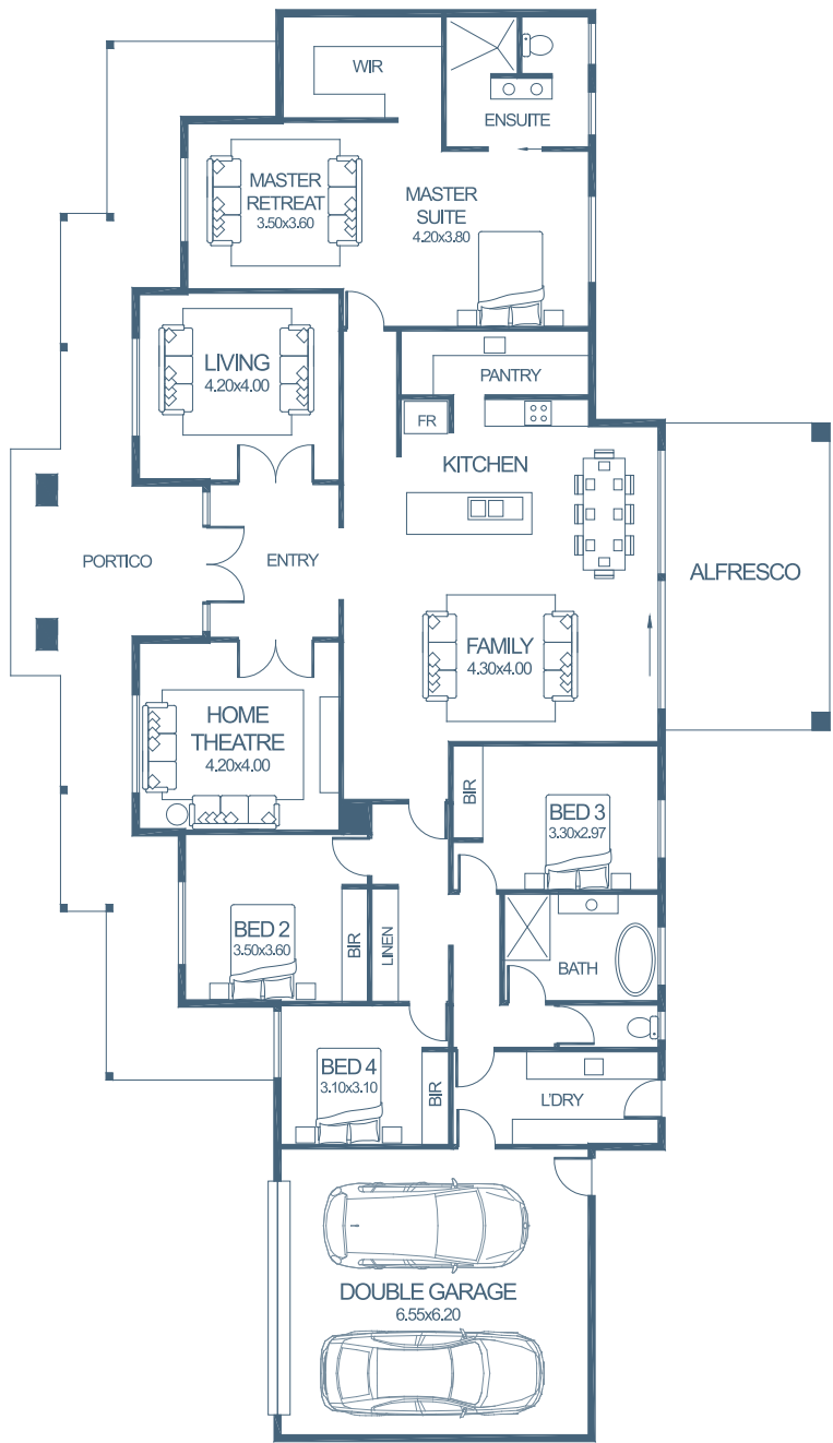
FLOORPLAN
